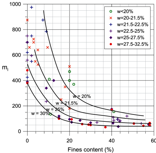
Figure 16.2. Modulus number for virgin loading as a function of fines content and water content.
