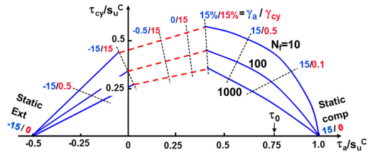
Figure 7.2. Contour diagram with number of cycles to failure as a function of average and cyclic shear stresses. Triaxial tests on normally consolidated Drammen Clay.
