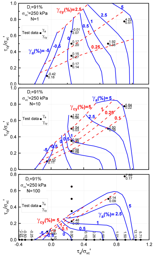
Figure 13.18. Average and cyclic shear strains as functions of average and cyclic shear stresses in triaxial tests on Sand 3. D_r \sim 91\% . w = 21\% . \sigma'_{vc} = 250 kPa. Precycling: 400 cycles of \tau_{cy}/\sigma'_{vc} = 0.1 . \Delta\tau_a applied drained by increasing vertical stress in compression and decreasing vertical stress in extension. Upper: N = 1 . Middle: N = 10 . Lower: N = 100 .
