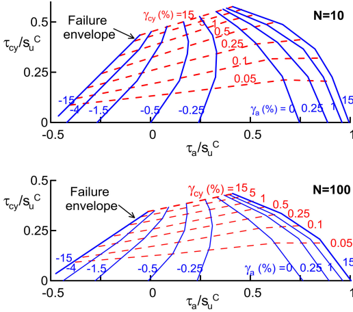
Figure 7.7. Average and cyclic shear strains after 10 and 100 cycles as functions of average and cyclic shear stresses. Triaxial tests on normally consolidated Drammen Clay.
