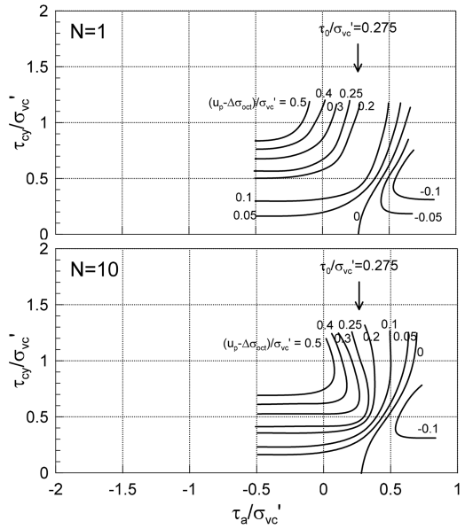
Figure 14.5. Permanent pore pressure as a function of average and cyclic shear stresses. Triaxial tests on Baskarp sand. D_r \sim 96\% . w = 20\% . \sigma'_{v,c} = 250 kPa. Precycling: 400 cycles of \tau_{cy}/\sigma'_{oct,c} = 0.1 . \Delta\sigma_a applied drained. Upper: N = 1 . Lower: N = 10 .
