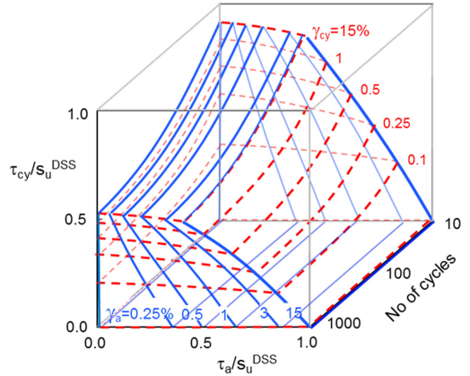
Figure 7.10. 3D representation of cyclic and average shear strains as functions of average and cyclic shear stresses and number of cycles. Normally consolidated Drammen Clay.
