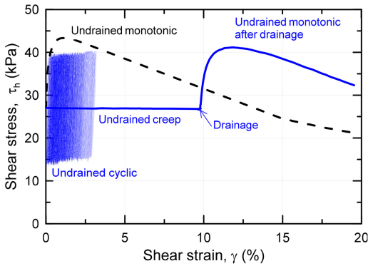
Figure 17.10. Effect of drainage after undrained cycling and creep on monotonic behavior of quick clay with \tau_a = \tau_c = 0.22 \cdot \sigma'_{vc} .
