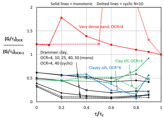
Figure 13.24. Secant shear modulus for overconsolidated relative to normally consolidated soils as a function of degree of shear strength mobilization. Undrained monotonic and two-way cyclic DSS tests.
