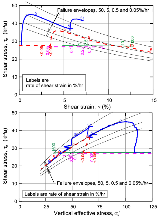
Figure 17.5. Stress-strain behavior (upper) and effective stress paths (lower) for creep and monotonic tests with different rate of shear strain. Quick clay with \tau_a = \tau_c = 0.22 \cdot \sigma'_{vc} .
