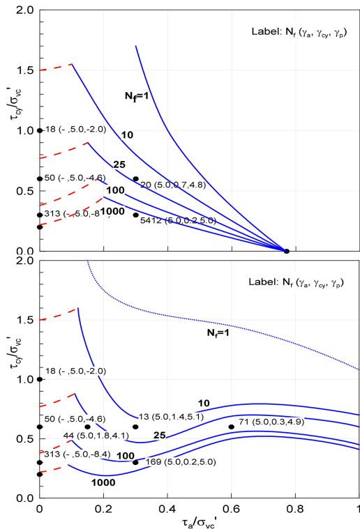
Figure 12.7. Cycles to “failure” ( \gamma = 5\% ) as a function of average and cyclic shear stresses. DSS tests. Normally consolidated very dense ( D_r \sim 105\% ) Dogger Bank sand. No fines. (Blaker & Andersen 2015). Upper: Drained \Delta\tau_a . Lower: Undrained \Delta\tau_a . \sigma'_{vc} = 200 kPa. Preshearing: 400 cycles at \tau_{cy}/\sigma'_{vc} = 0.06 .
