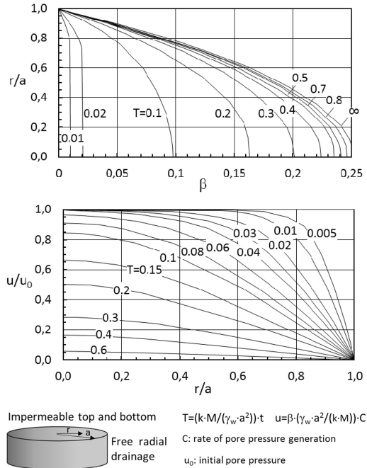
Figure 8.6. Dissipation of pore pressure in circular disk with radial drainage. Left: Pore pressure generated at constant rate (based on Heiberg 1973), Right: Initial pore pressure u = u_0 in entire volume at t = 0 (based on Madhus & Hårvik 1988).
