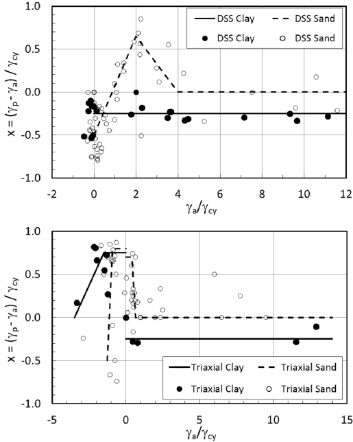
Figure 7.8. Relationship between permanent and average shear strains for normally consolidated Drammen clay and dense sand ( D_r \sim 80 to 100\% ). Undrained loading. Upper: DSS. Lower: Triaxial.
