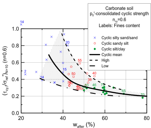
Figure 12.43. Cyclic shear strength of p'_0 -consolidated non-cemented carbonate soils in DSS tests with \tau_a = 0 as a function of water content.
