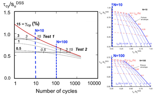
Figure 7.9. Cyclic shear strain as a function of cyclic shear stress and number of cycles in DSS tests with \tau_a = 0 on normally consolidated Drammen Clay.
