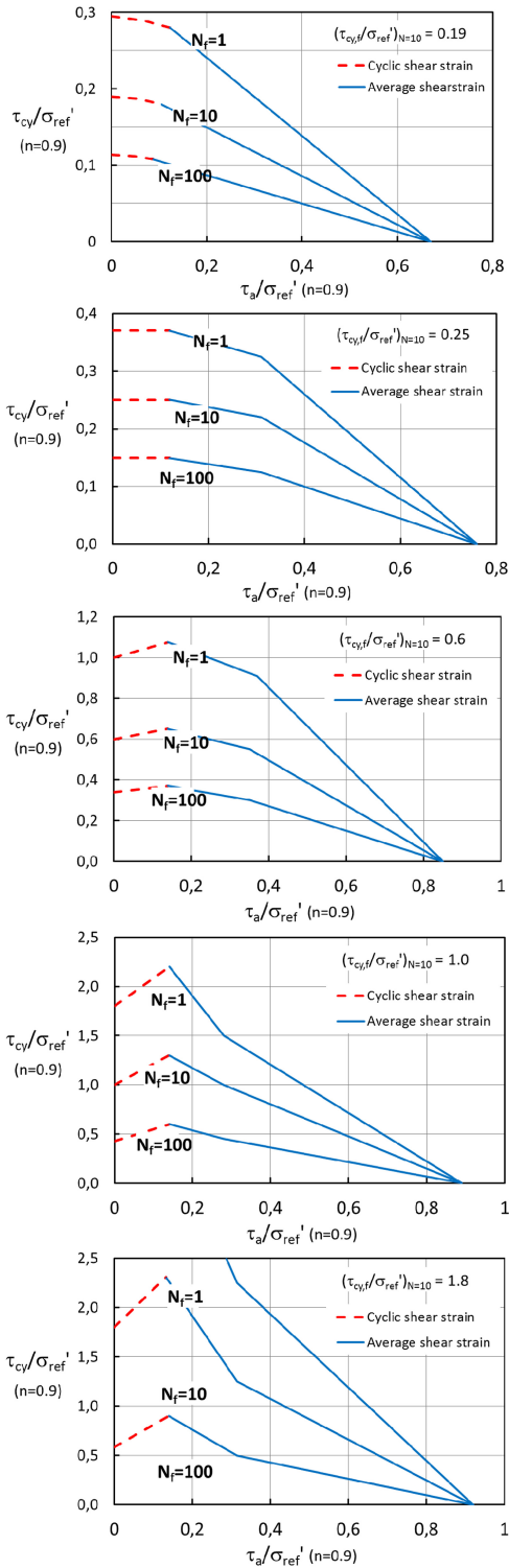
Figure 12.16. Combination of average and cyclic shear stresses that cause failure as a function of number of cycles. DSS tests on normally consolidated sand and silt with different (\tau_{cy,f}/\sigma'_{ref})_{N=10} for \tau_a = 0 . \tau_a applied drained.
