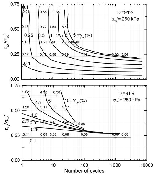
Figure 13.13. Average (upper) and cyclic (lower) shear strains as functions of N and \tau_{cy}/\sigma'_{vc} for \tau_a/\sigma'_{vc} = \tau/\sigma'_{vc} = 0.25 in triaxial tests on Sand 3. D_r \sim 91\% w = 21\% . \sigma'_{vc} = 250 kPa. Precycling: 400 cycles of \tau_{cy}/\sigma'_{vc} = 0.1 . Prepared by pluviation.
