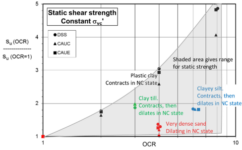
Figure 10.7. Undrained static shear strengths as a function of OCR.
