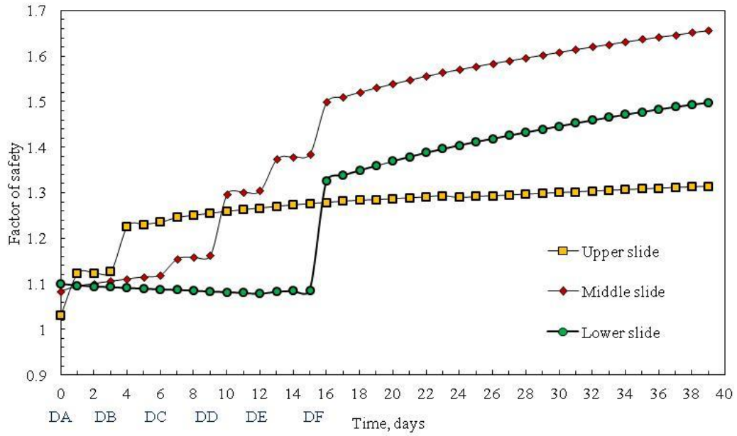
Figure 5.14 Variation of factor of safety of three slides under Case 2 - top down
