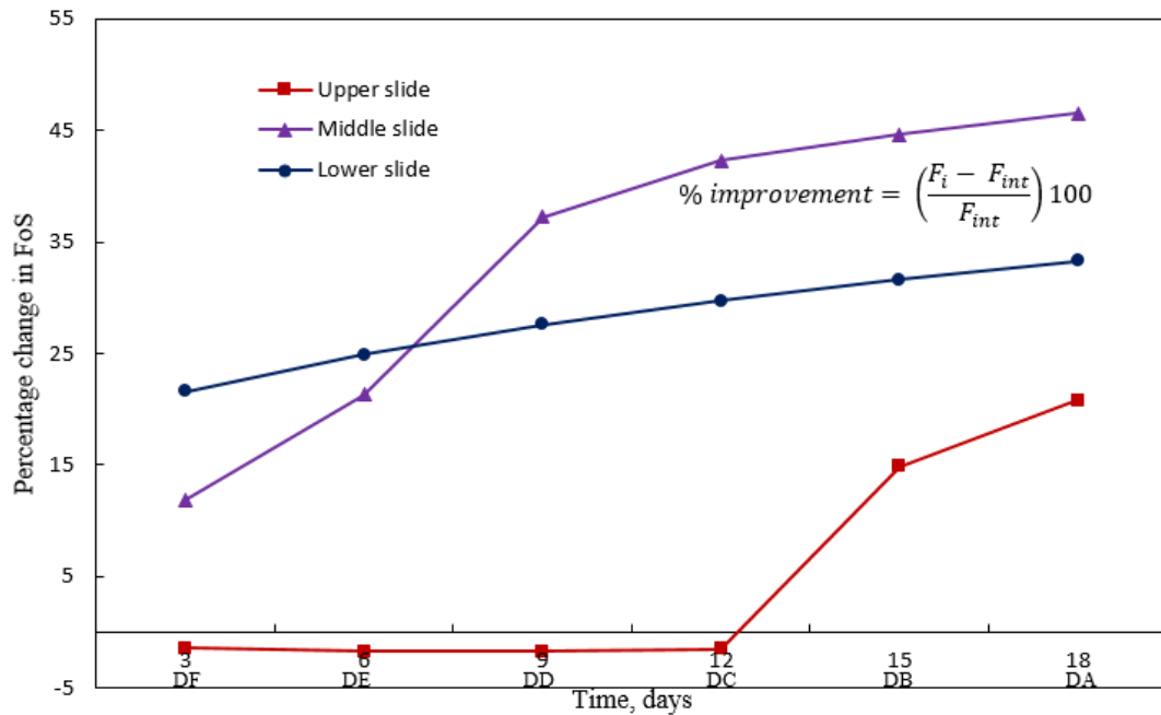
Figure 5.17 Percentage Improvement in factor of safety of each slide under sequential construction in Case 3 - bottom up
