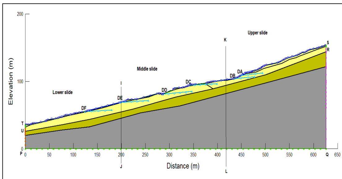
Figure 5.10 Drains simulated in the section A1 - A2
