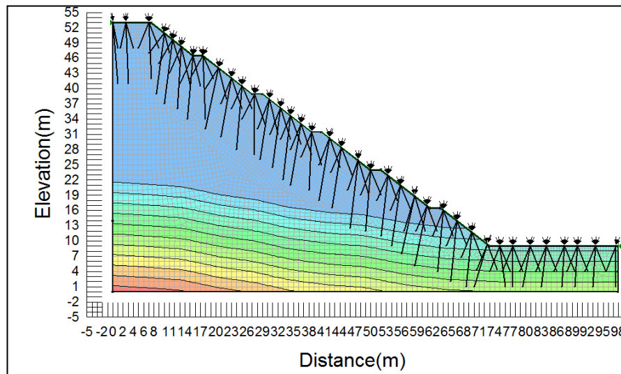
Figure 2.45 Root configuration used in the analysis (Dharmasena et al., 2015)
