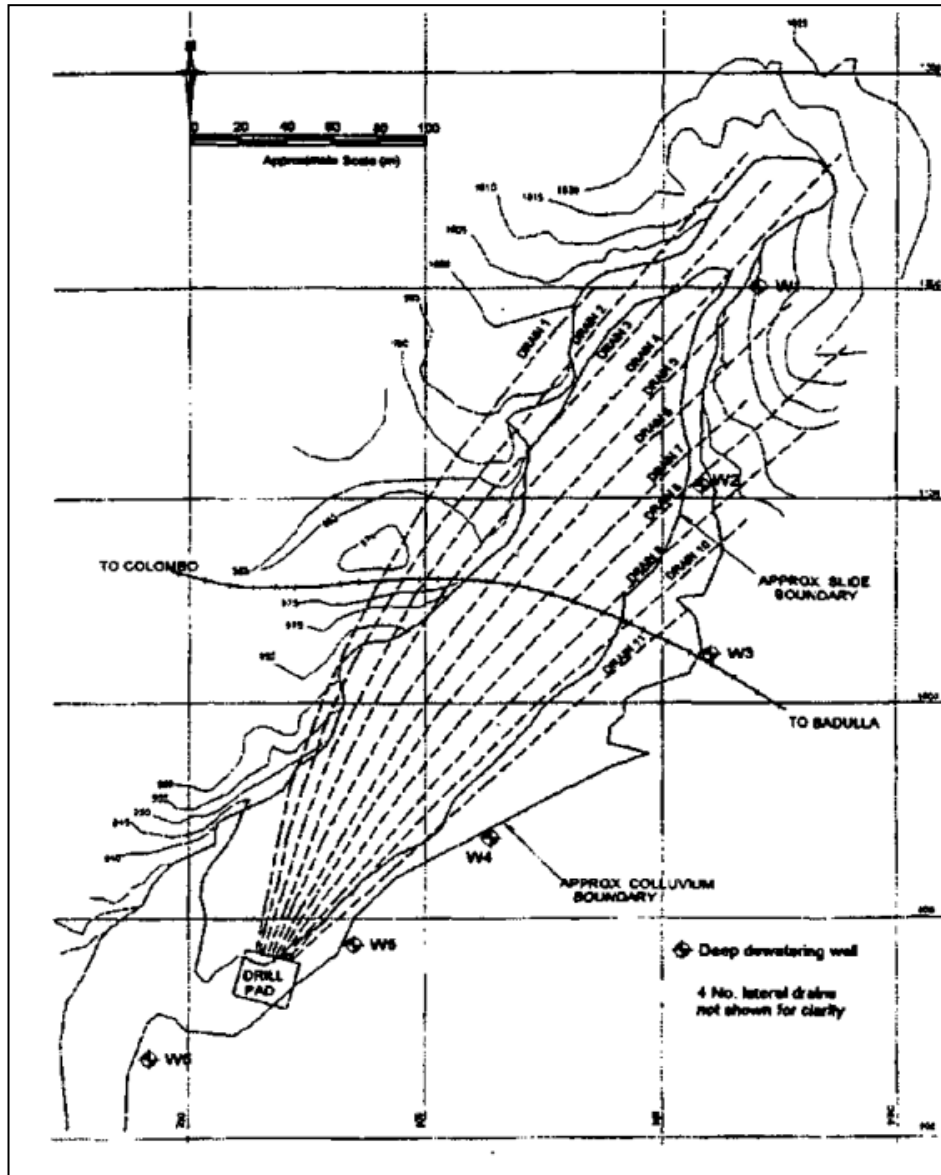
Figure 2.18 Layout of subsurface drains and deep wells at Watawala landslide (Chandler and Broise, 2000)
