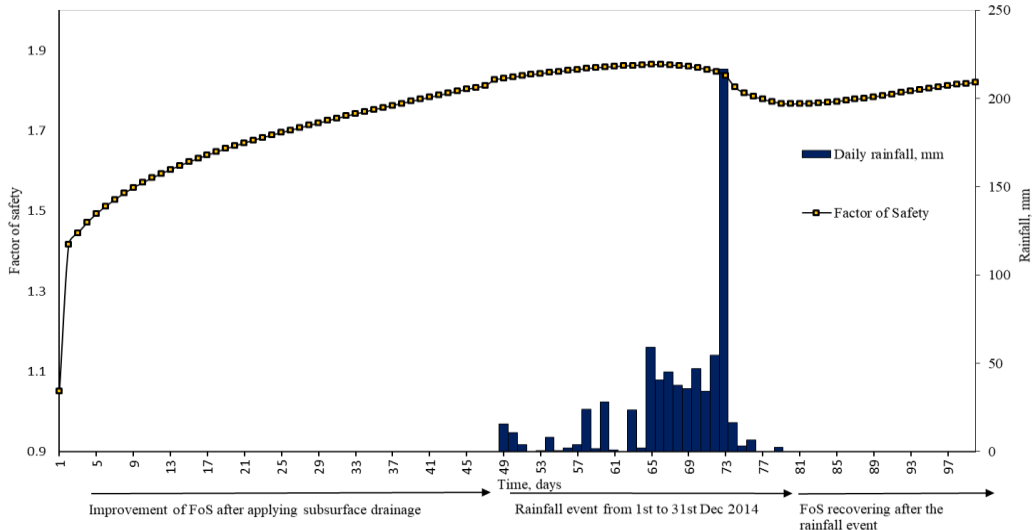
Figure 5.30 Variation of the factor of safety after implementing hybrid mitigation measures, corresponding to an actual rainfall event
