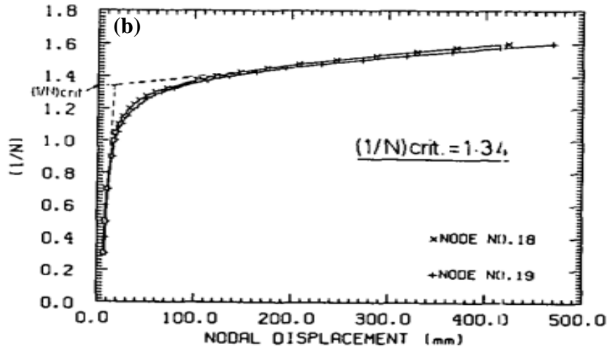
Figure 2.7 (a): A homogeneous simple slope composed of two soil layers (b): Nodal displacement curves obtained for the slope at Nodes 18 and 19 (Donald and Giam 1988)
