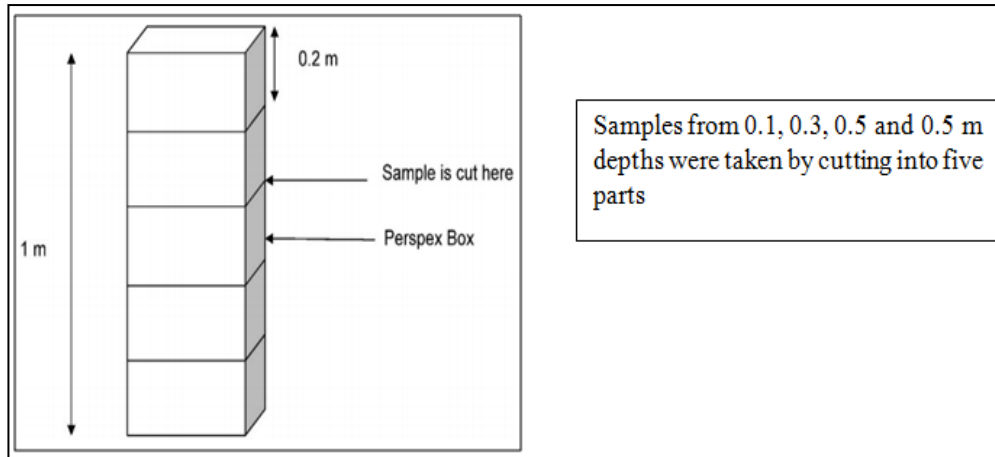
Figure 2.32 Perspex boxes for preparation of samples (Ali and Osman 2008)
