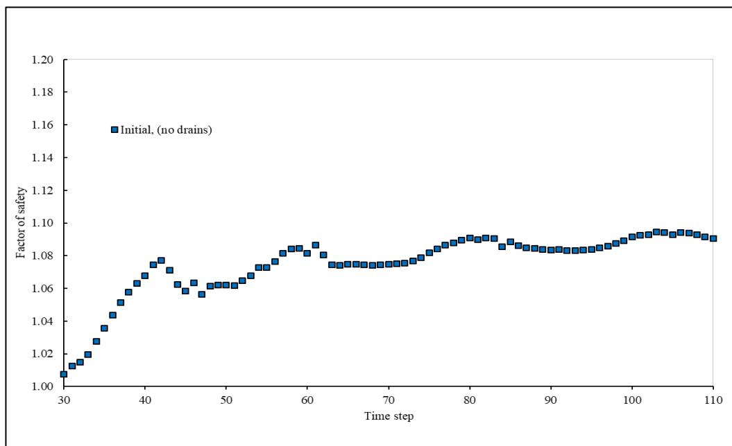
Figure 6.11: Plot showing the initial factor of safety of the slope
