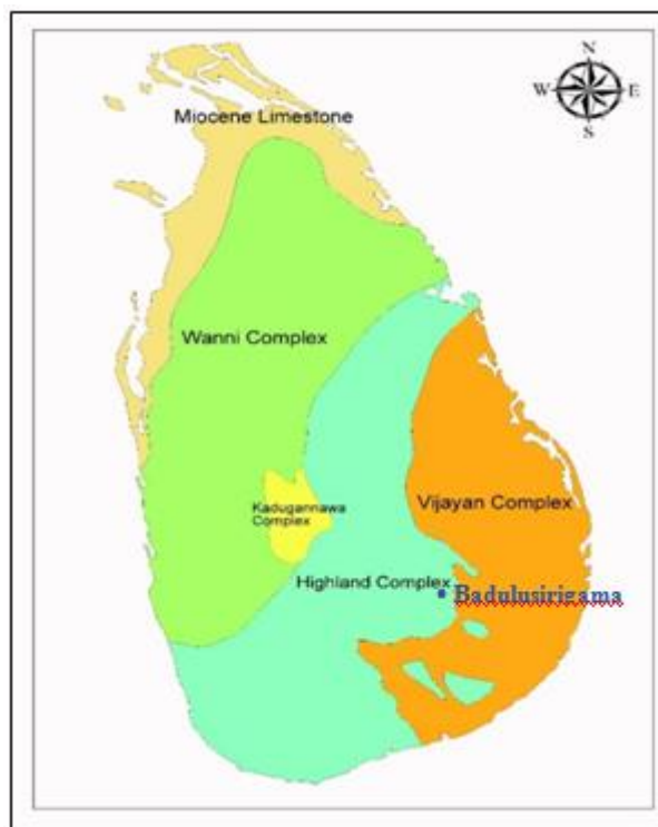
Figure 3.3 Geological complexes of Sri Lanka and location of Badulusirigama site
