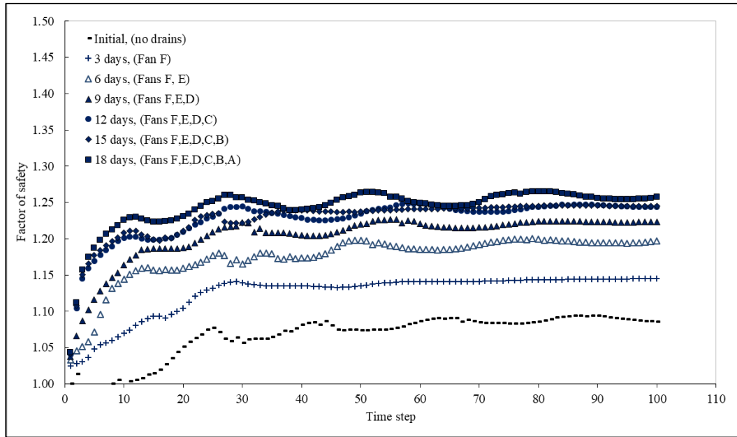
Figure 6.16: Variation of factor of safety pertaining to Case 3
