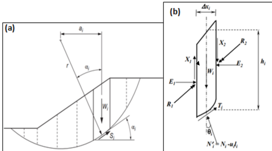
Figure 2.3: (a) Circular slip surface with overlying soil mass subdivided into slices (Duncan et al., 2014), (b) Forces acting on a slice
