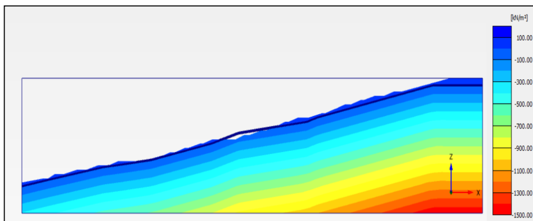
Figure 6.5 Variation of the pore water pressure along the section PQ
