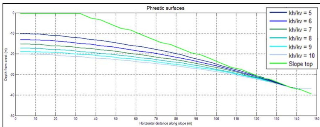
Figure 2.10 Modelled phreatic surfaces for a slope with no drains with different anisotropic ratios of permeability (Pathmanathan 2009)
