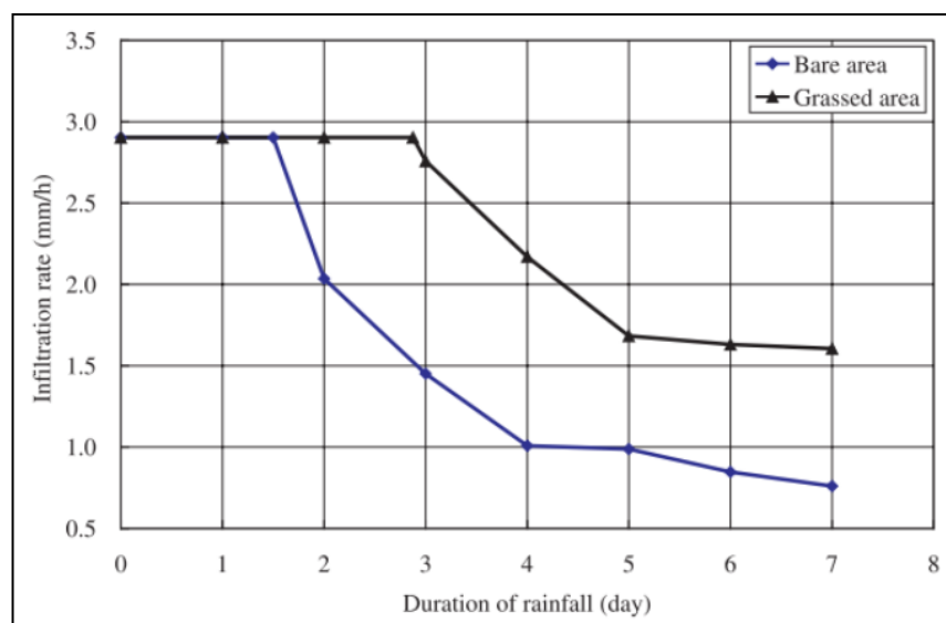
Figure 2.42 Rate of infiltration into a bare area and a vegetated area of slope (Zhan et al., 2007)
