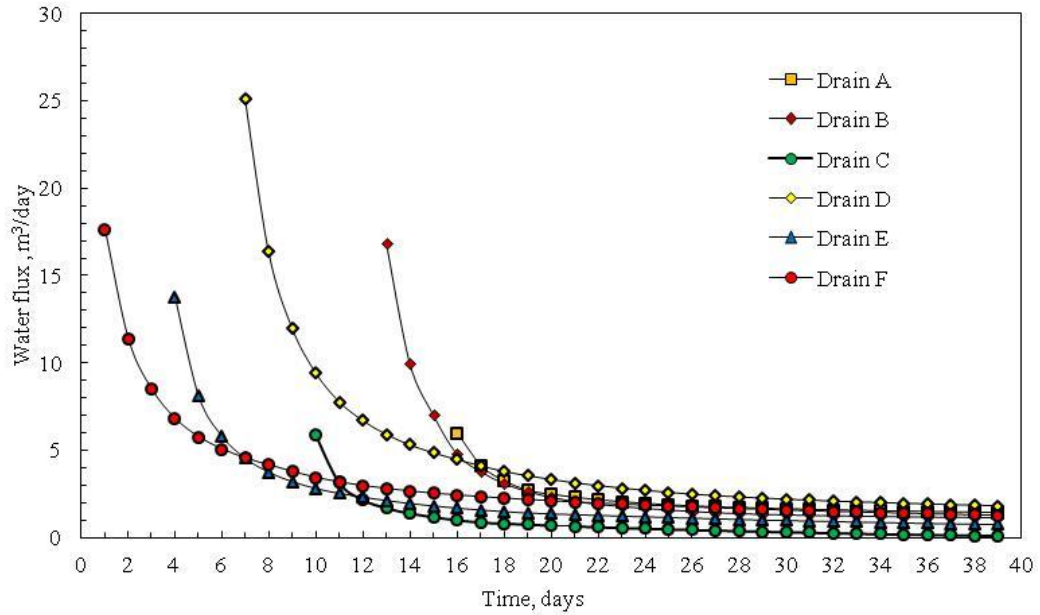
Figure 5.13 Comparison of the water flux into the drains for Case 3
