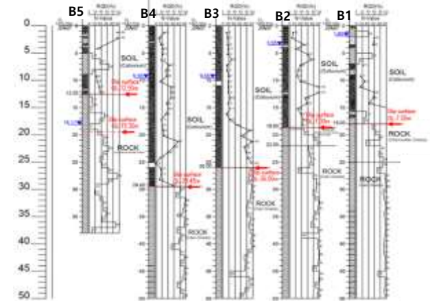
Figure 6. Identified slip surface using output of borehole investigation
