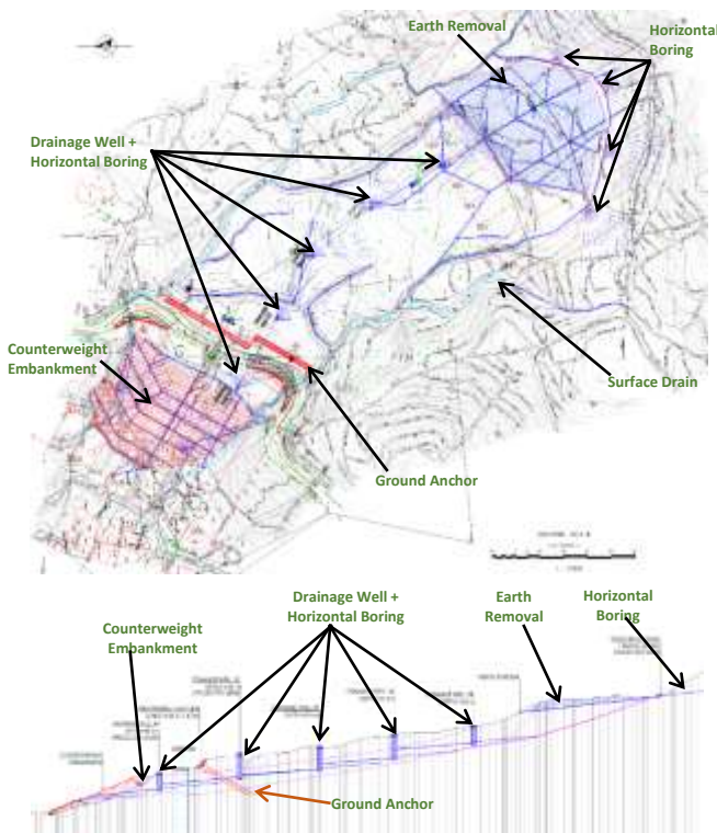
Figure 12. Plan view and cross section of proposed countermeasures
