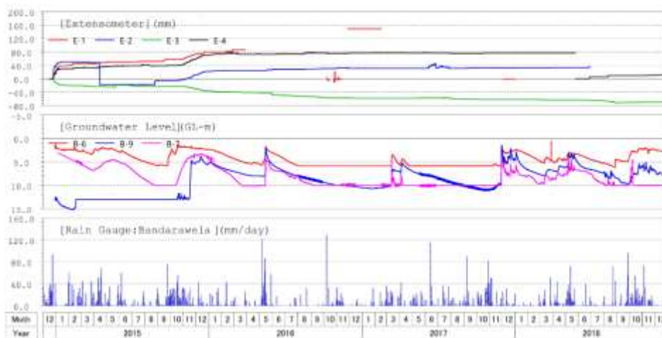
Figure 4. The response of water level meter and extensometer for the rainfall received
